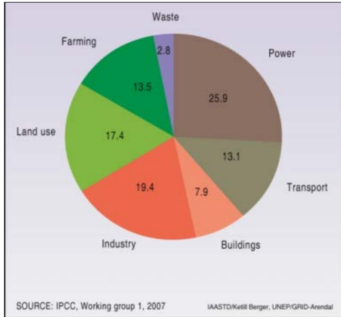
GHG emissions by source as a percentage of total GHG emissions (2004)
